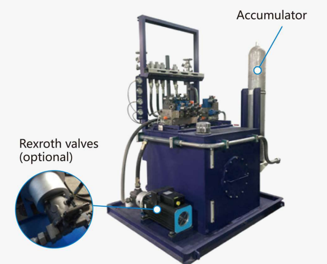
Ordinary type hydraulic system
